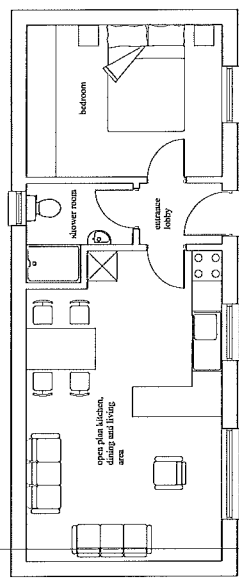
Proposed Plan 1:50
